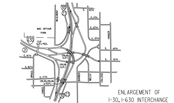
ENLARGEMENT OF CLINTON AVE. INTERCHANGE
