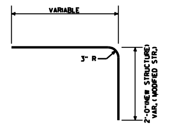
DETAIL OF BENT "b" BAR
